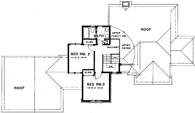
SECOND FLOOR PLAN LIVING AREA: 516 SQ. FT.
