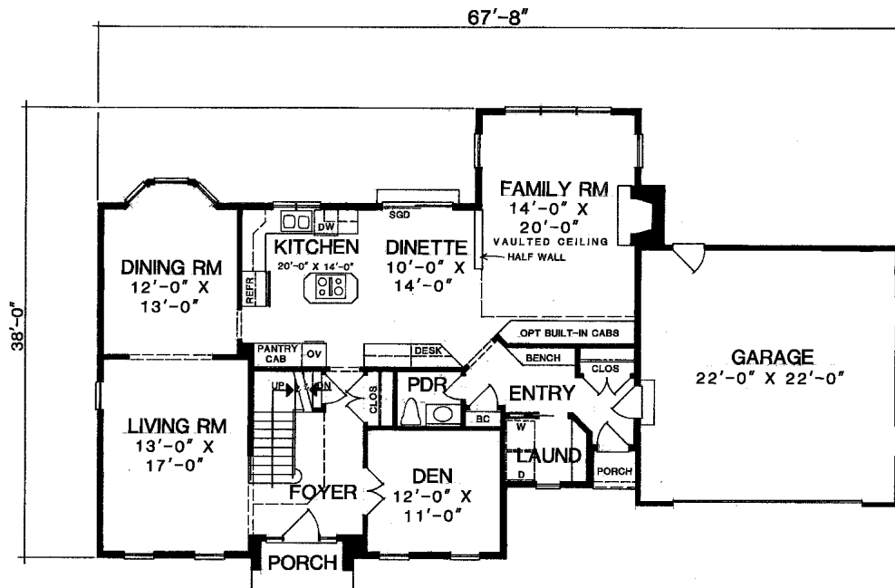
FIRST FLOOR PLAN LIVING AREA: 1413 SQ FT
